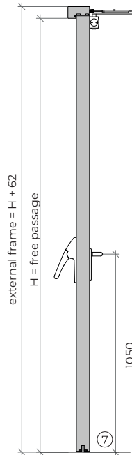
vertical section
