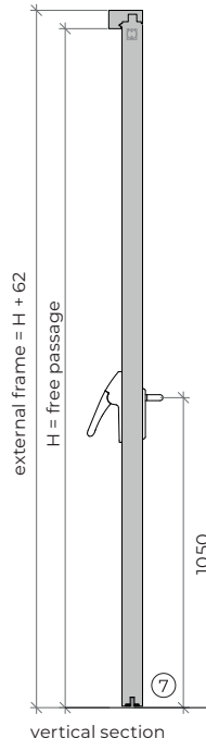
vertical section
