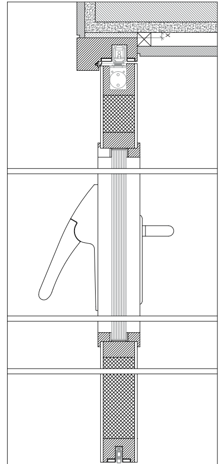
standard frame | hidden door closer | concrete wall mounting | fixation with expandable foam | plaster and wood finishes
