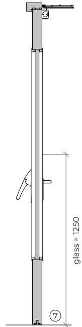
vertical section
