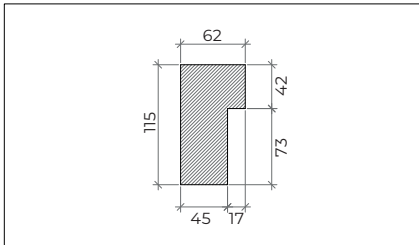
standard frame | hidden hinges | concrete wall mounting | fixation with expandable foam | plaster and wood finishes
