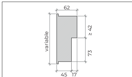
modified frame | visible hinges | concrete wall mounting | fixation with expandable foam | plaster and wood finishes
