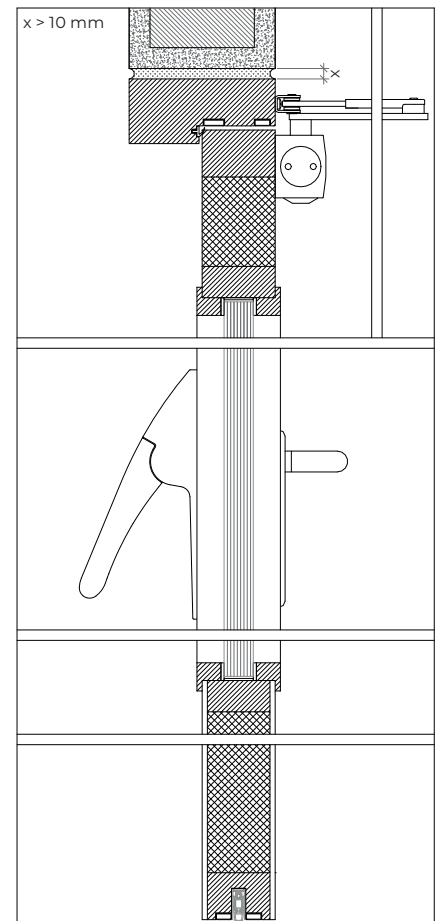
modified frame | door closer with articulated arm | concrete wall mounting | fixation with expandable foam
