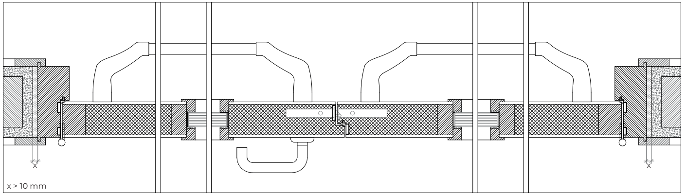
modified frame | visible hinges | concrete wall mounting | fixation with expandable foam | plaster and wood finishes
