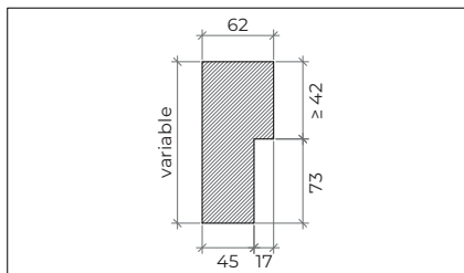
modified frame | visible hinges | concrete wall mounting | fixation with expandable foam
