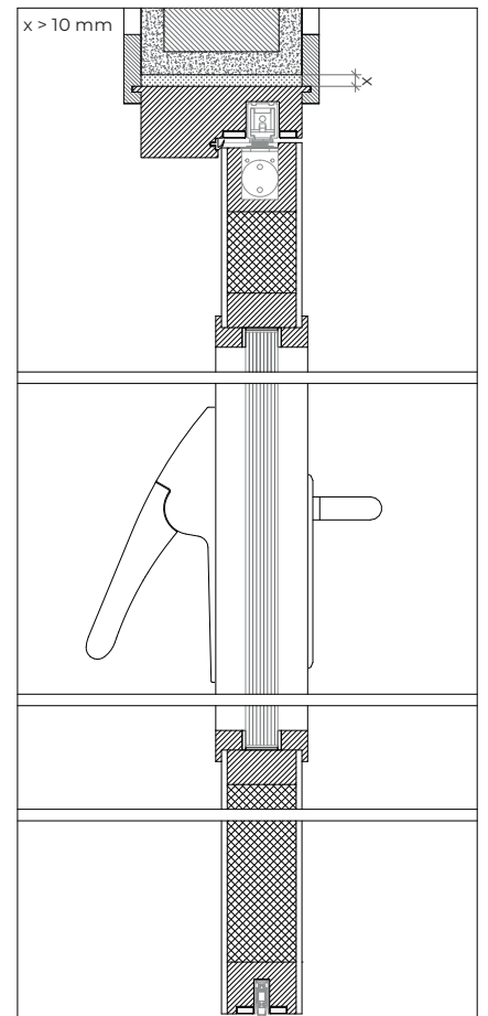
modified frame | hidden door closer | concrete wall mounting | fixation with expandable foam | plaster and wood finishes
