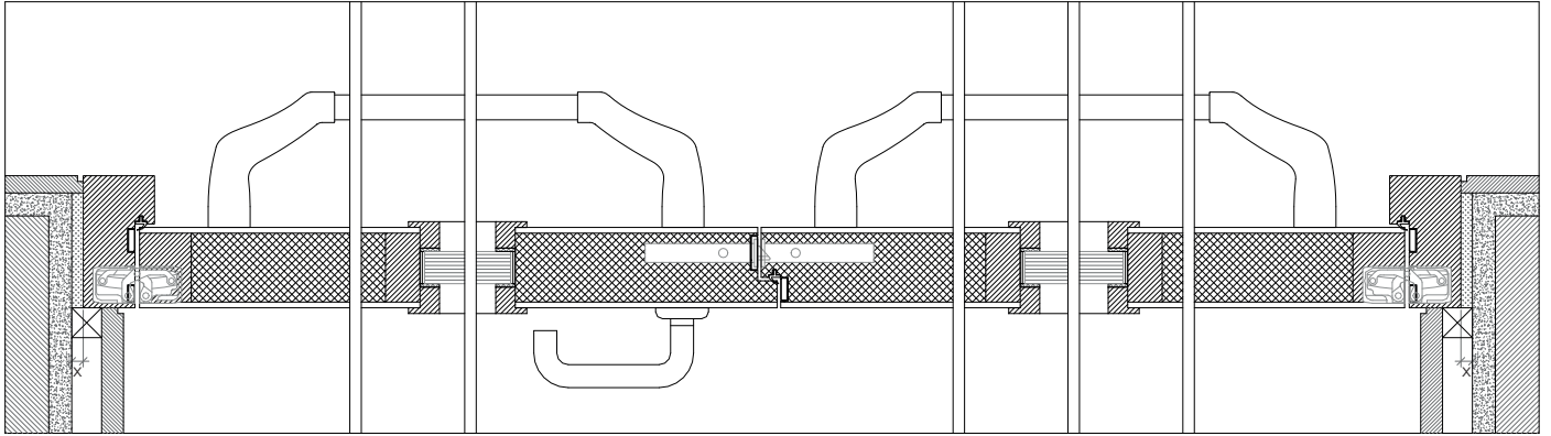
standard frame | hidden hinges | concrete wall mounting | fixation with expandable foam | plaster and wood finishes
