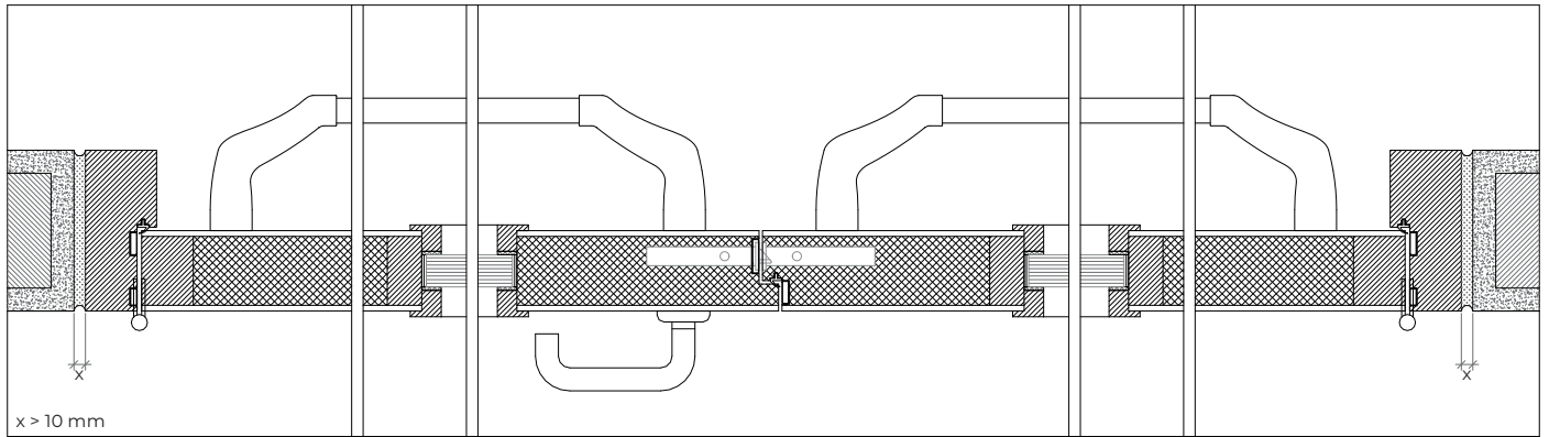
modified frame | visible hinges | concrete wall mounting | fixation with expandable foam
