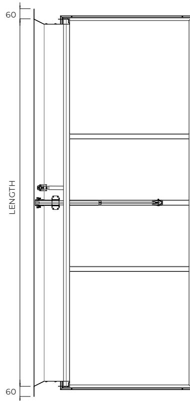
SECTION B-B
