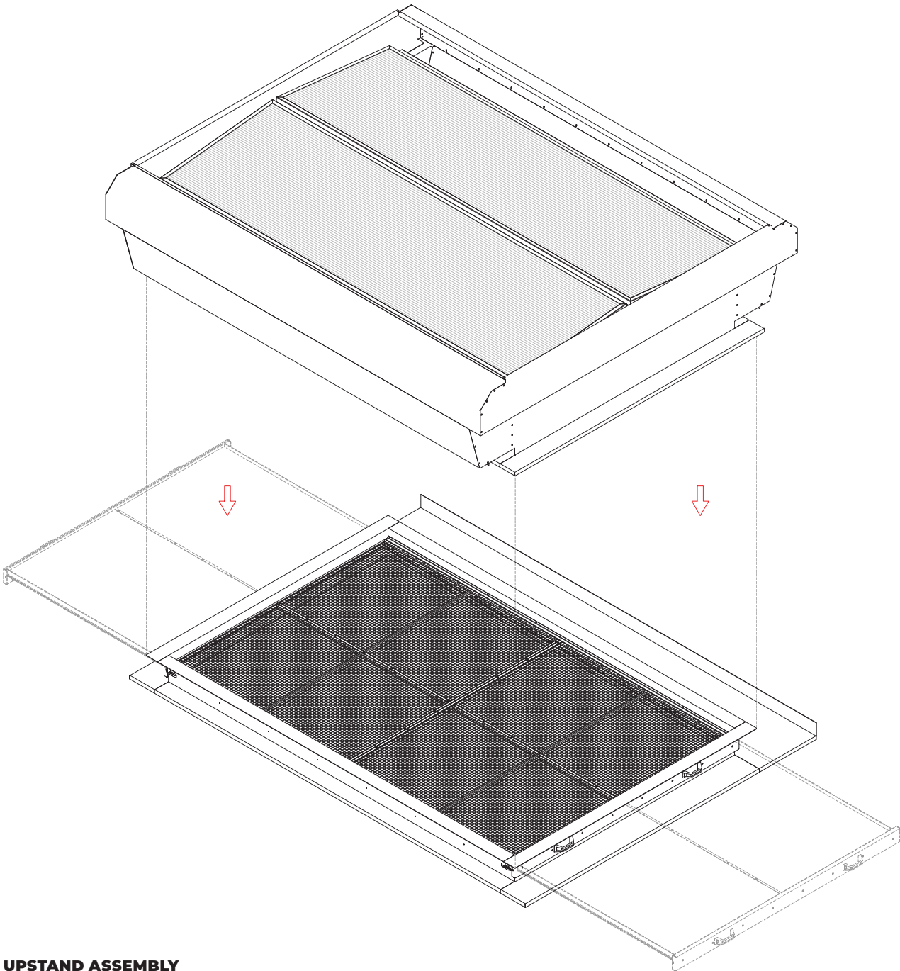
UPSTAND ASSEMBLY
