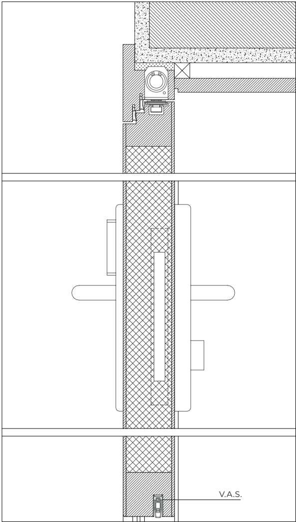
ceiling aligned with the door frame | inverted door closer to allow adjustment from the frame: solution approved up to EI2 45
