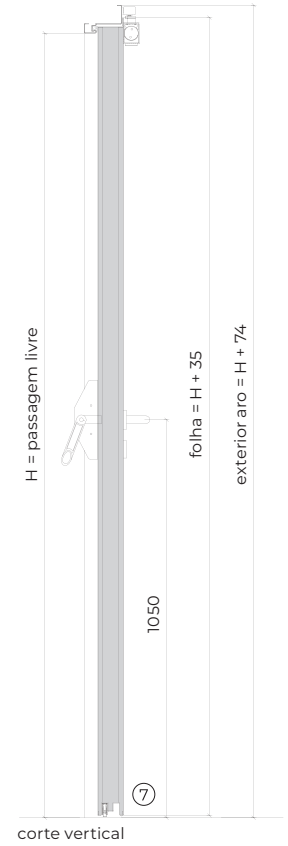
corte vertical
